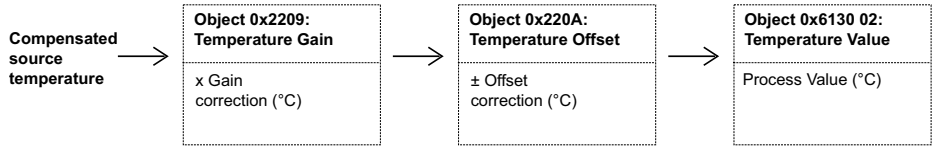
Figure 8: Temperature Calibration Offset
