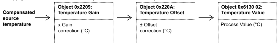
Figure 7: Temperature Calibration Gain
