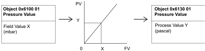
Figure 9: Scale of Pressure and Temperature Output
